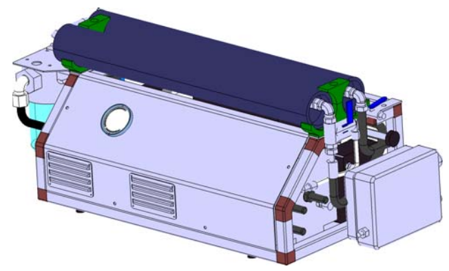
ISO VIEW Scala: 1:10
